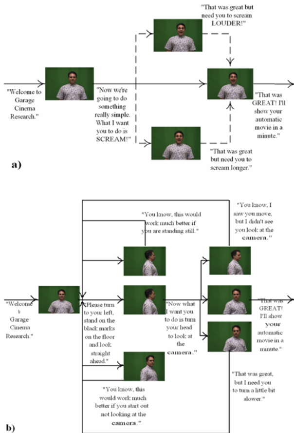
Figure 1. Active Capture process for capturing (a) “Scream” shot and (b) “Head Turn” shot. (Quotes are verbal instructions from the Active Capture system. The continuously horizontal left-to-right arrows represent an error-free path. The other arrows are error correction loops.)
